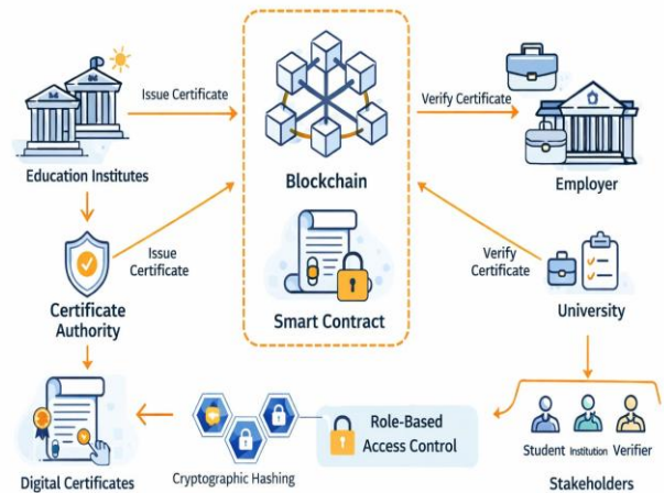
Fig. 1: Workflow of VerifyCerts Diagram
