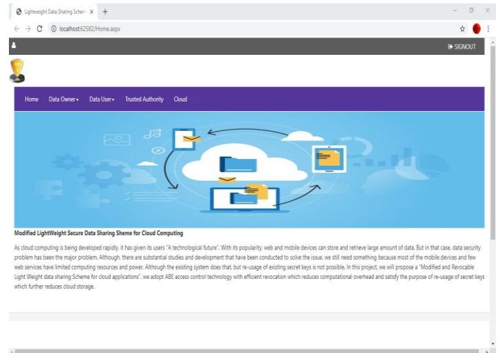
Fig 2: Home Page
