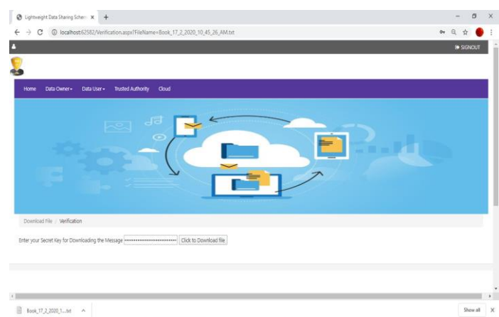
Fig 10: Download File
