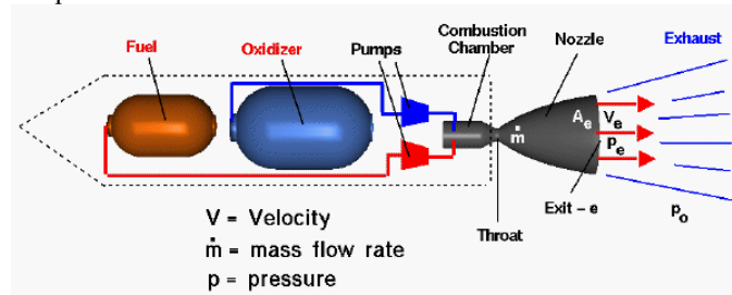
Fig. 4. Liquid propellant rocket engine.
