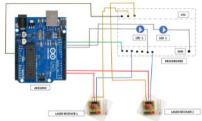
Fig.1. Circuit Diagram
