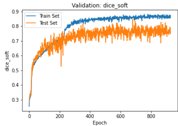
Figure 17 Validation Loss of Our Model CV-3
