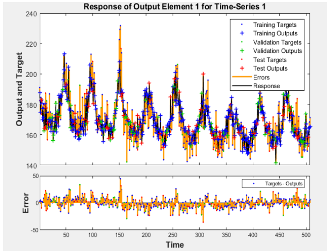
Fig 15: Time Series Response of NIO
