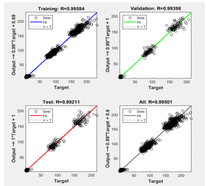
Fig 14: Regression of NIO plot (plotregression).
