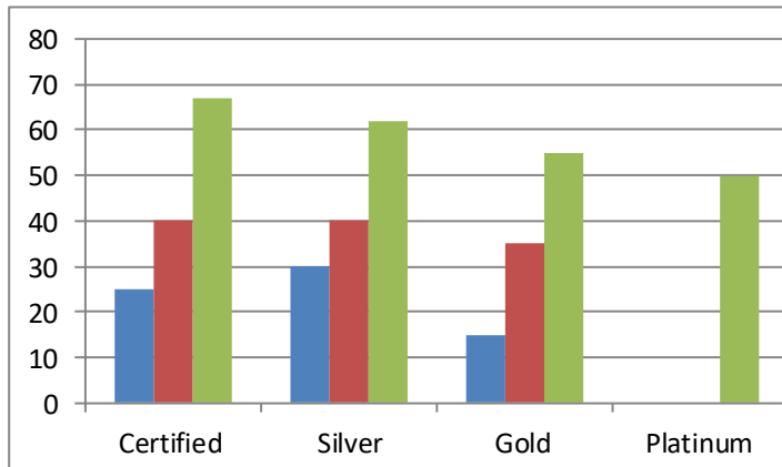
Fig. 2 -ENERGY USE BY LEED CERTIFICATION – Self analyzed
