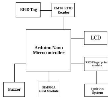
Fig. 1 Block diagram of the system.
