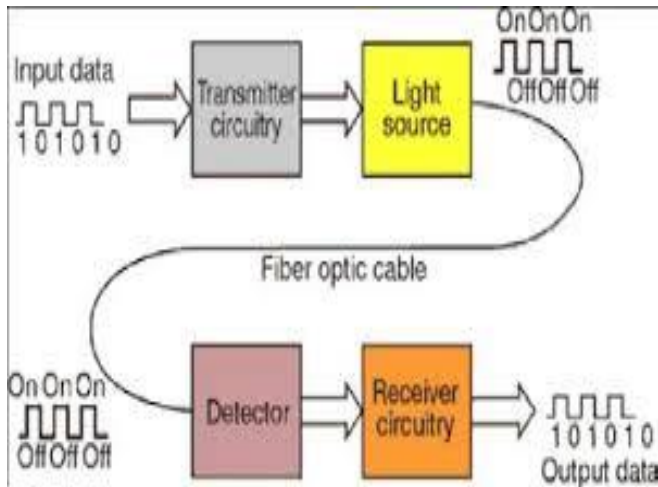
Fig.1. Basic fiber optic communication system [5]
