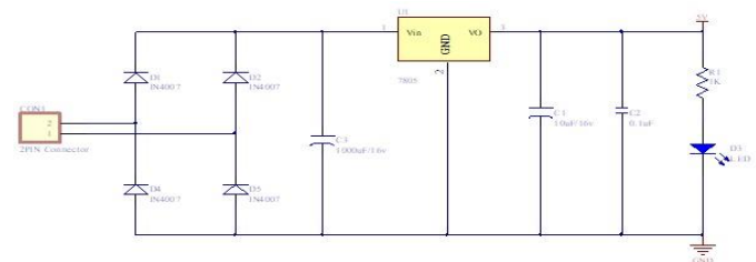
Fig. 5 Power Supply Design
