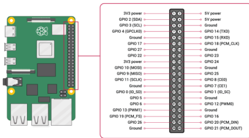
Fig. 2. Pinout
