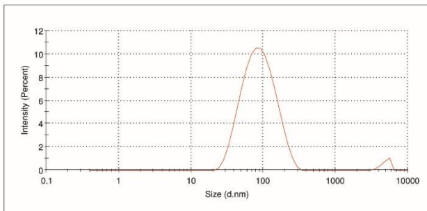
Fig. 2 DLS image of Alumina nanoparticles
