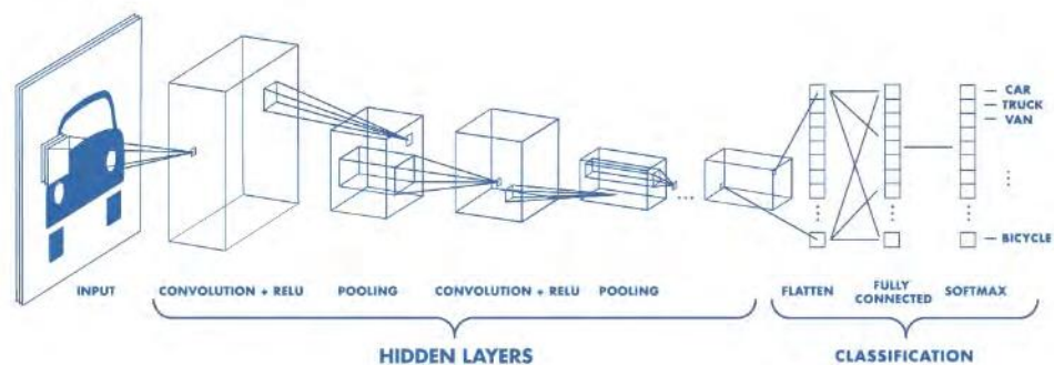
Fig. 3.6 Schematic representation of a Convolutional Neutral Network. (Source: “Introduction to Deep Learning: What Are Convolutional Neural Networks?”)
