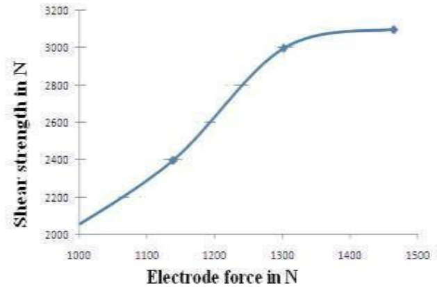
Fig.4 Electrode force Vs shear strength
