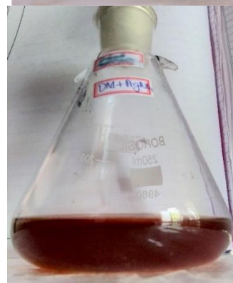
Before reduction of Ag 2+ (pale yellow) after reduction of Ag 2+ (reddish brown)
